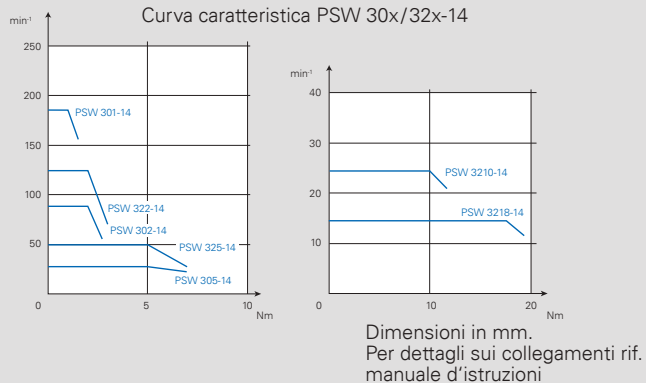
Curva caratteristica PSW 30x/32x-14
