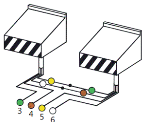
2 x 2-wire cable
