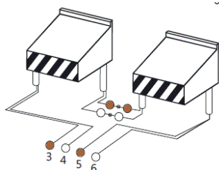
2 x 2-wire cable
